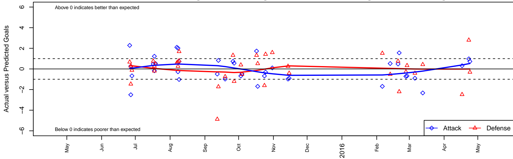
CSC Storm Navy G03 Dots are actual minus expected GF (blue circles) and GA (red triangles). Blue line is smoothed change in attack strength. Red is smoothed change in defense strength.
